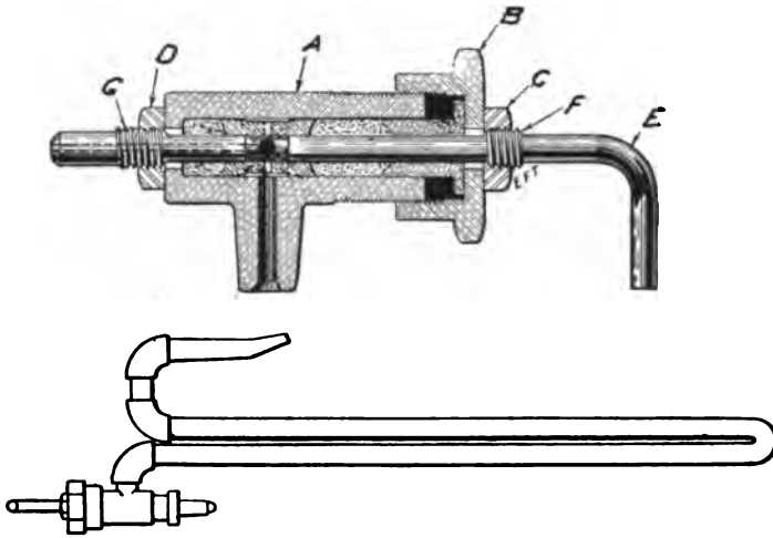
FIG. 217.—Usual pattern of "torch" head and starting "torch," used on several American steam carriages. The head parts are lettered as follows: A, body of head; B, threaded cap; C and D, nuts working on screws, F and G, on rod, E. Screw, G, gives attachment to the collar on the valve stem, as shown at B, in the succeeding figure.
